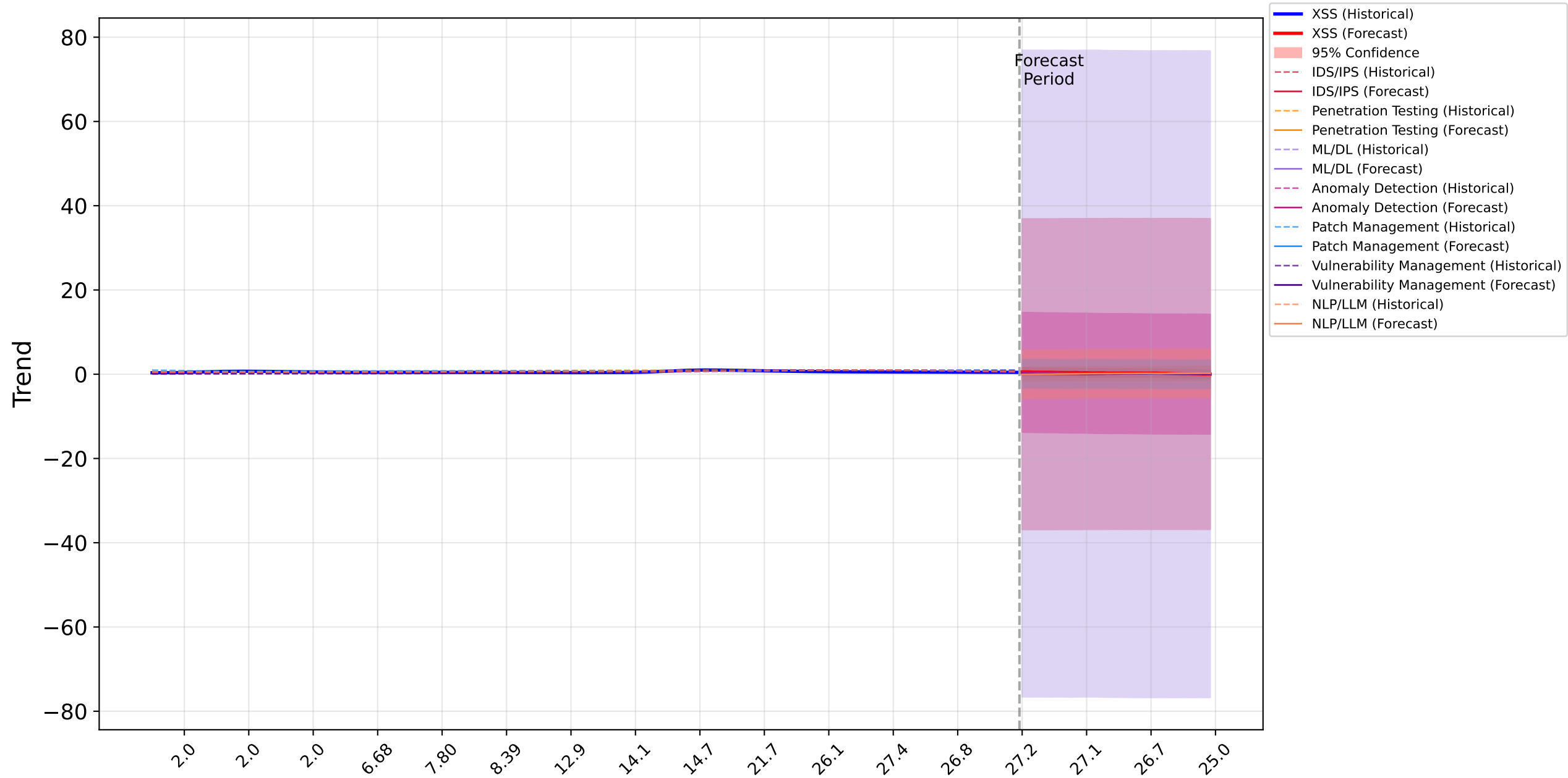
XSS Forecast Historical: 2.0 to 22.53454696505373 | Forecast: 2025-01 to 2027-12
